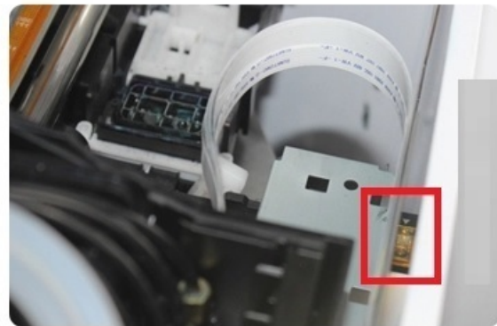
Photoelectric sensor
